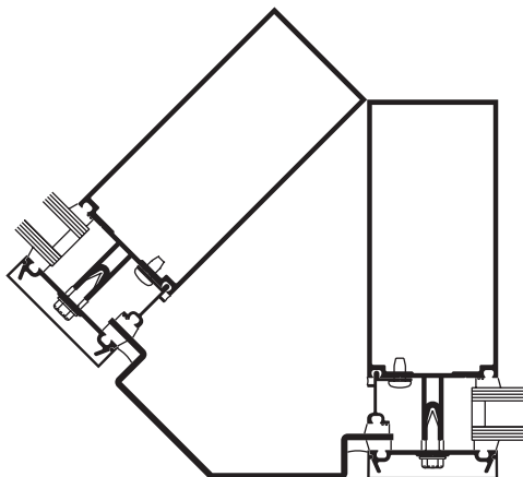
135° OUTSIDE CORNER
