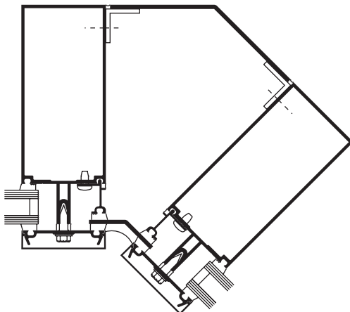
135° INSIDE CORNER
